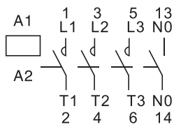
CJX2-0910Z~3210Z
