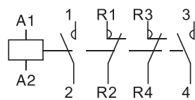
CJX2-09008Z~25008Z
