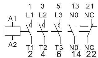
CJX2-4011Z~9511Z
