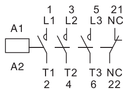
CJX2-0901Z~3201Z
