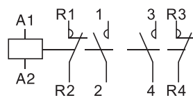
CJX2-40008Z~95008Z
