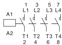
CJX2-09004Z~32004Z
